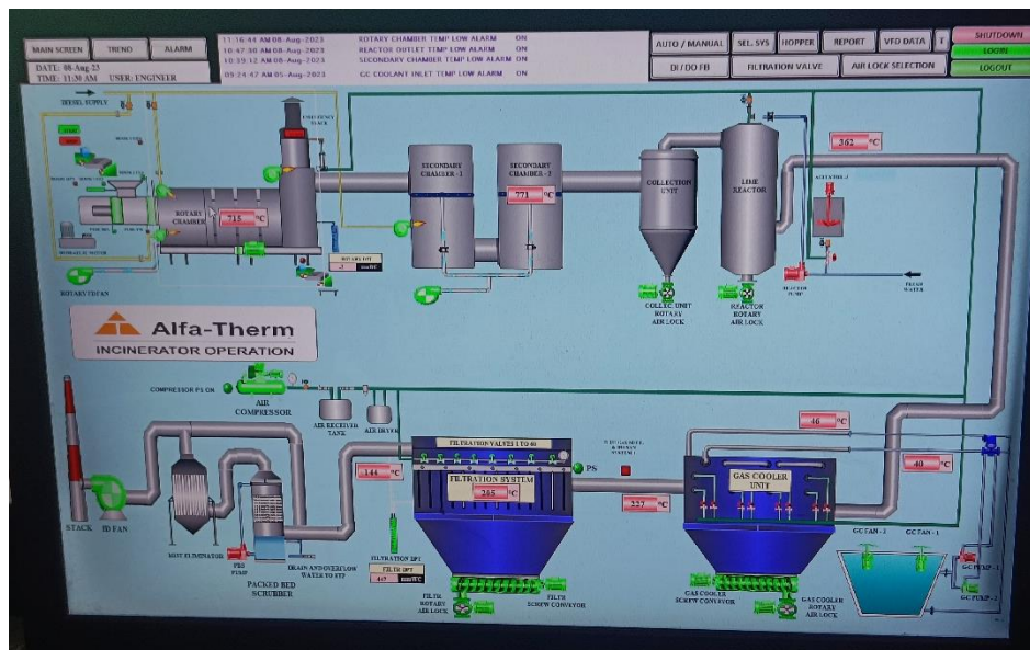
New Rotary (Dry Scrubber) – Plant No.1
